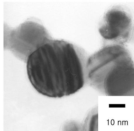
Fig. 2. TEM observation results show Ni synthesized using WF.
