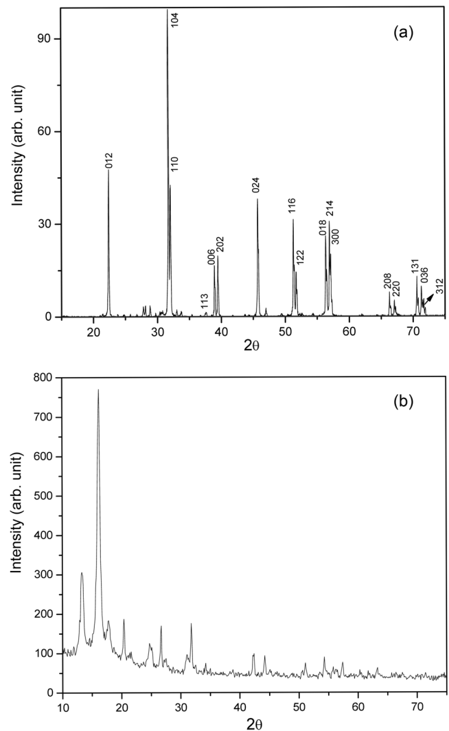
Fig. 1. (a) XRD patterns of \text{BiFeO}_3 sintered at 880\text{ }^\circ\text{C} . (b) XRD patterns of \text{BiFeO}_3 sintered at 860\text{ }^\circ\text{C} .
