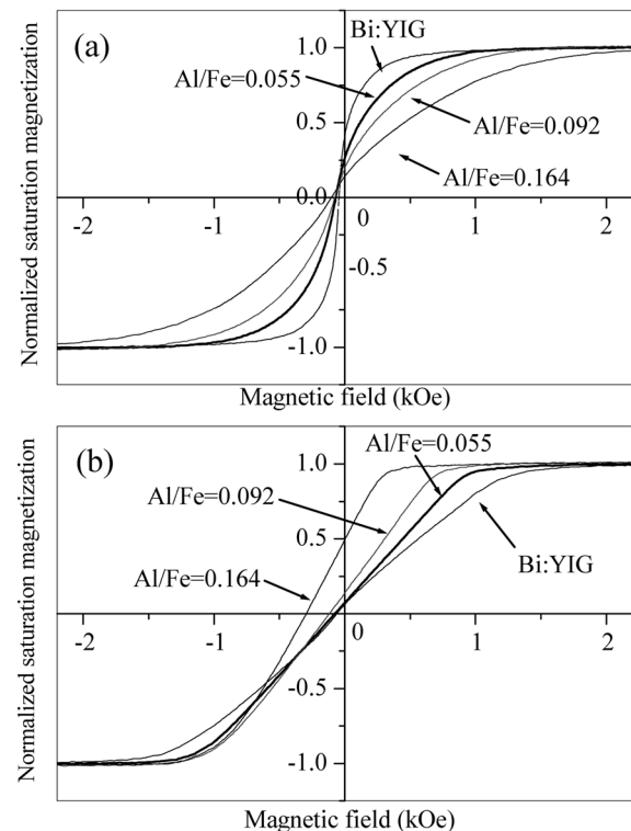
Fig. 4. Magnetization curves normalized by saturation magnetization for (a) in-plane and (b) out-of-plane directions.
