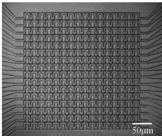
Fig. 5. Photograph of the fabricated multiple-tone MO-SLM.
