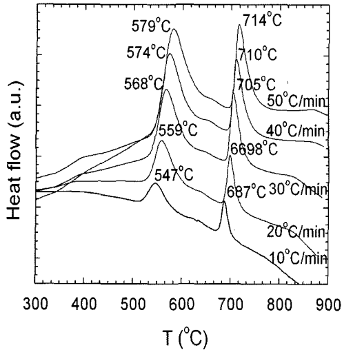
Fig. 2. The DSC curves of as-quenched \text{Fe}_{73.5}\text{Si}_{13.5}\text{B}_9\text{Nb}_3\text{Au}_1 alloy with different heating rates (from 10^\circ\text{C}/\text{min} to 50^\circ\text{C}/\text{min} ).
