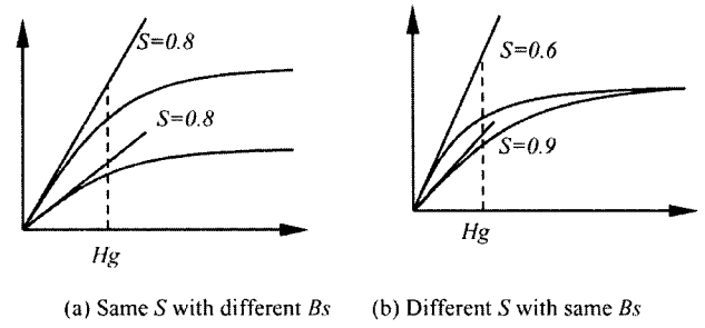
Fig. 7. Two types of B-H curves and saturation factors.
