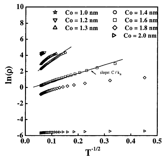
Fig. 5. \ln(\rho) vs. T^{-1/2} for the samples of [\text{AlN}(3\text{ nm})/\text{Co}(t\text{ nm})]_{10}/\text{AlN}(3\text{ nm}) multilayers having different Co-layer thickness. The activation energy C \approx 12.8\text{ meV} for \text{Co} = 1.4\text{ nm} and 2.3\text{ meV} for \text{Co} = 1.6\text{ nm} , respectively.
