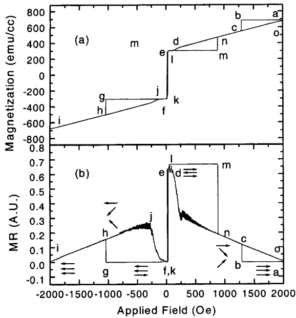
Fig. 8. (a) M-H and (b) MR-H hysteresis loops for a cell size of 16 \mu\text{m} \times 8 \mu\text{m} at a maximum applied field of 2000 Oe, which is above the threshold field for magnetization flop. The results are obtained for H_{\text{bias}} = 26 Oe, H_{\text{Py}} = 5 Oe, H_{\text{anti}} = -1000 Oe, H_{\text{Co}} = 20 Oe, and H_{\text{pin}} = 0 . The magnetic configurations at some important points during the field cycle are also illustrated in (b).
