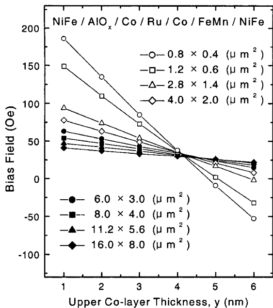
Fig. 2. Bias field as a function of the relative Co-layer thickness in the SyAF for various cell sizes.
