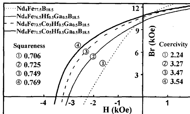
Fig. 6. Demagnetization curves of Nd_4Fe_{76.5-x}Co_xHf_{0.5}Ga_{0.5}B_{18.5} melt spun ribbons annealed at 680 °C for 10 min.
