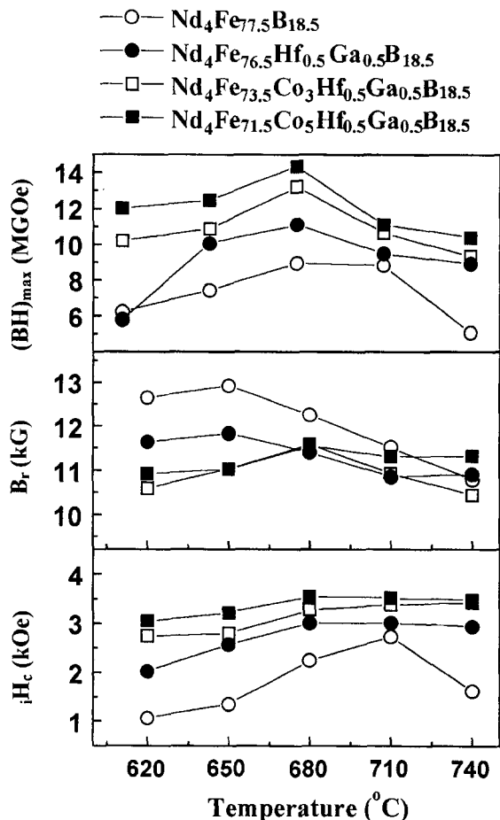
Fig. 5. Magnetic properties of Nd_4Fe_{76.5-x}Co_xHf_{0.5}Ga_{0.5}B_{18.5} ribbons melt spun at a wheel speed of 26 m/sec as a function of annealing temperature.
