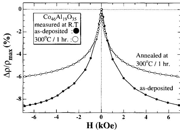
Fig. 8. Magnetoresistance curves for the as-deposited and 300°C-1 hour annealed \text{Co}_{46}\text{Al}_{19}\text{O}_{35} granular thin film.
