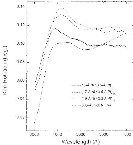
Fig.6. Typical Kerr spectra of Ni/Pt multilayers corresponding to (15-Å Ni/3.5-Å Pt) 15 , (17-Å Ni/3.5-Å Pt) 15 , and (19-Å Ni/3.5-Å Pt) 15
