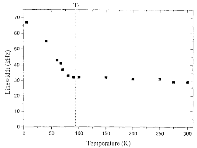
Figure 2. Temperature dependence of the 19 F NMR linewidth.
