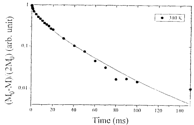
Figure 3. The 19 F nuclear magnetization recovery pattern at 310 K in the fluorinated YBa 2 Cu 3 O 7-x .
