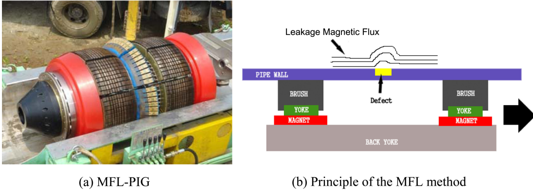
Fig. 1. (Color online) MFL PIG and the principle of the MFL method [2].
