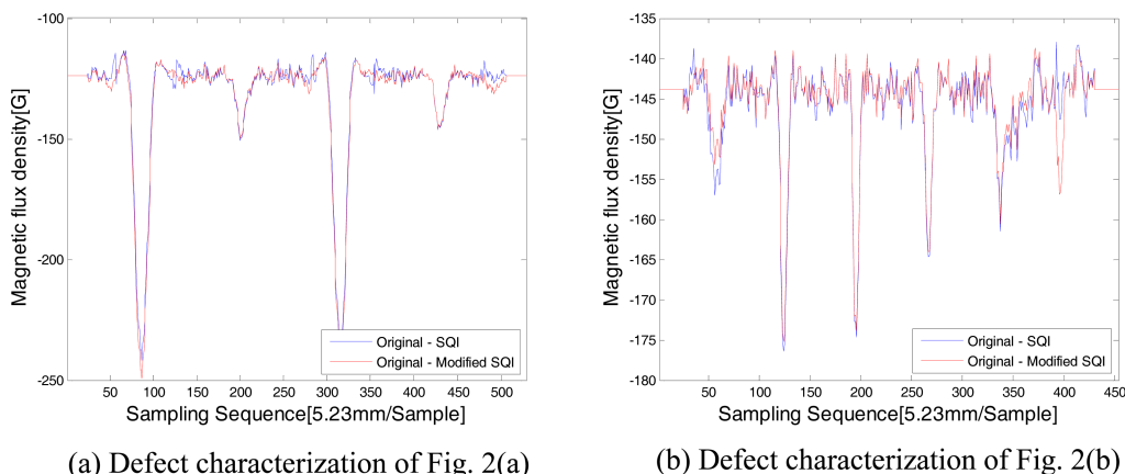
Fig. 3. (Color online) Preprocessed signals using SQI and the modified SQI.
