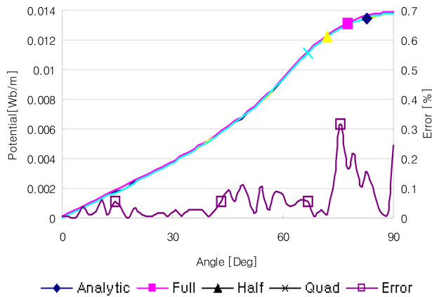
Fig. 9. (Color online) Potential comparison along the test path.
