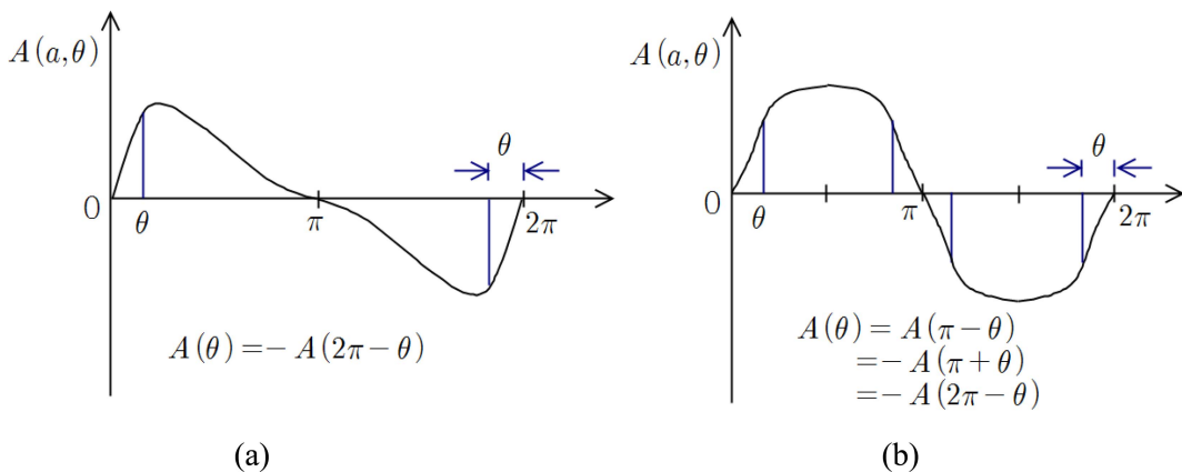
Fig. 3. (Color online) Potential distributions of symmetrical and periodic structure.
