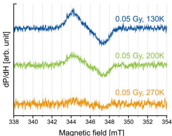
Fig. 4. (Color online) EPR spectra of the 0.05 Gy-irradiated tris sample according to temperature.
