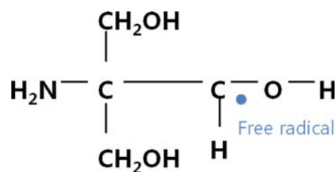
Fig. 2. (Color online) The molecular structure and electron free radical of irradiated-tris.
