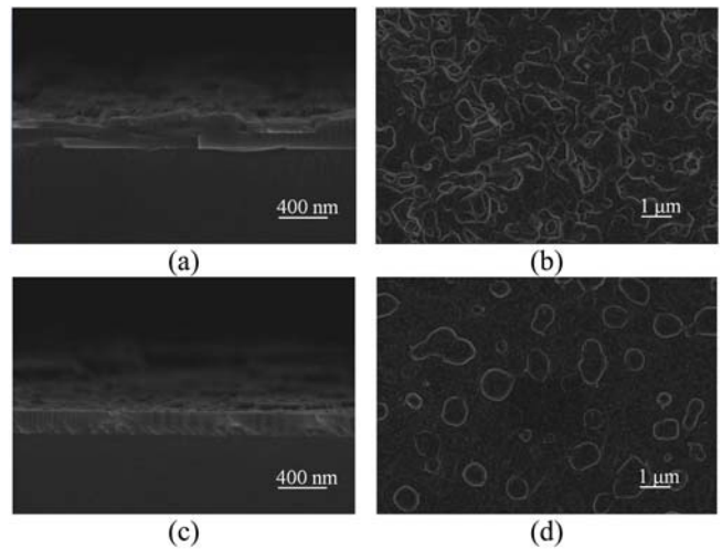
Fig. 4. Shows the cross-sectional and surface morphology of 9 ml-added YBCO films that were heat treated from 755 to 800 °C after calcining at 400 °C; [(a), (b)]: 755 °C, and [(c), (d)] 800 °C.
