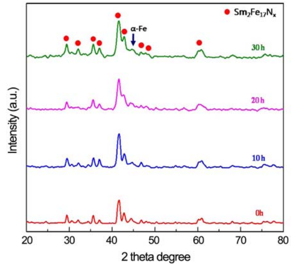
Fig. 5. XRD patterns of Sm 2 Fe 17 N x powders before and after ball milling for 10, 20, and 30 hours.
