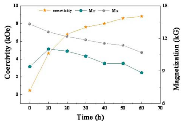
Fig. 6. Dependence of the magnetic properties of Sm 2 Fe 17 N x powders on the ball milling time.
