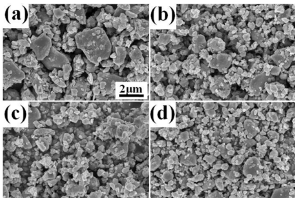
Fig. 4. Typical SEM images of Sm 2 Fe 17 N x powders after ball milling for 10, 30, 50, and 60 hours.
